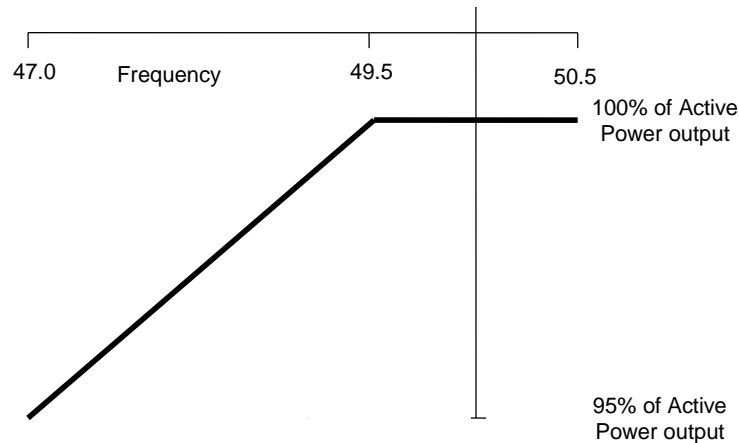
Figure 2 – Change in output power with falling frequency
