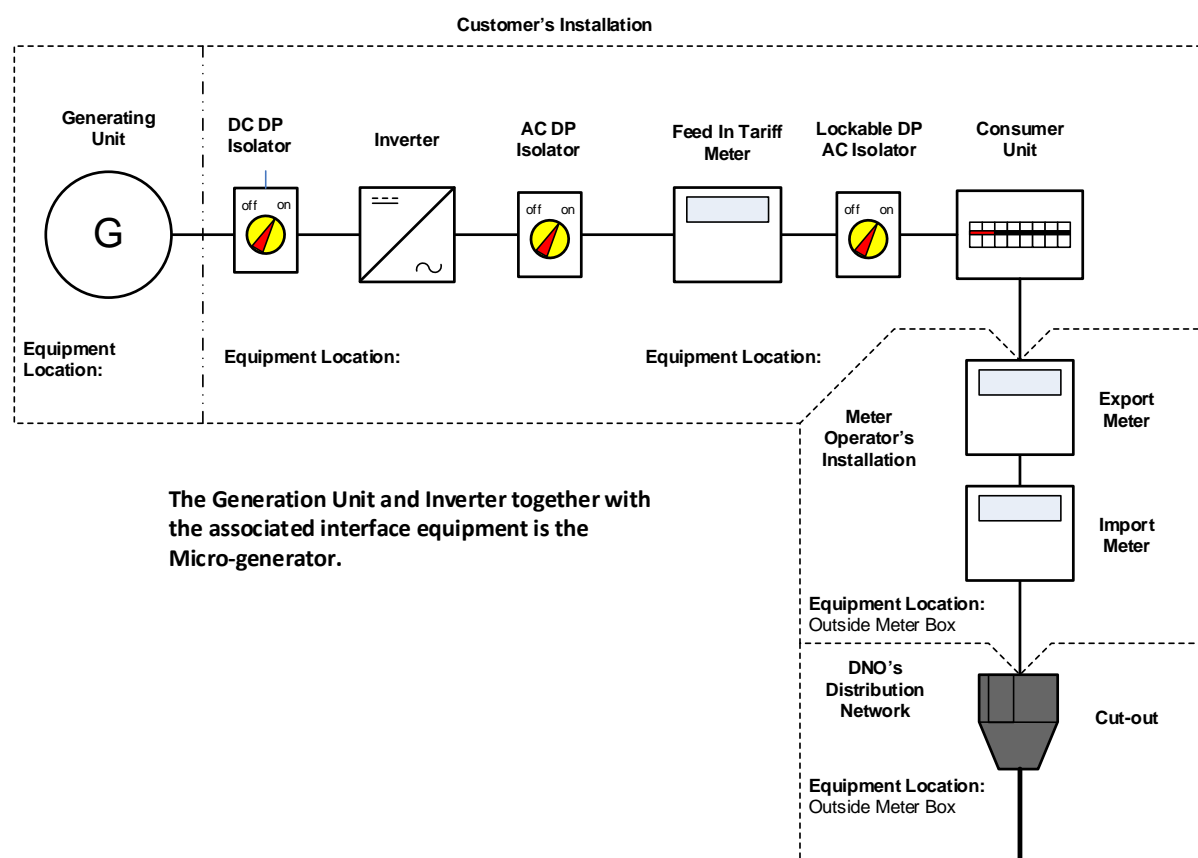
Figure 1 – Example of the type of circuit diagram
