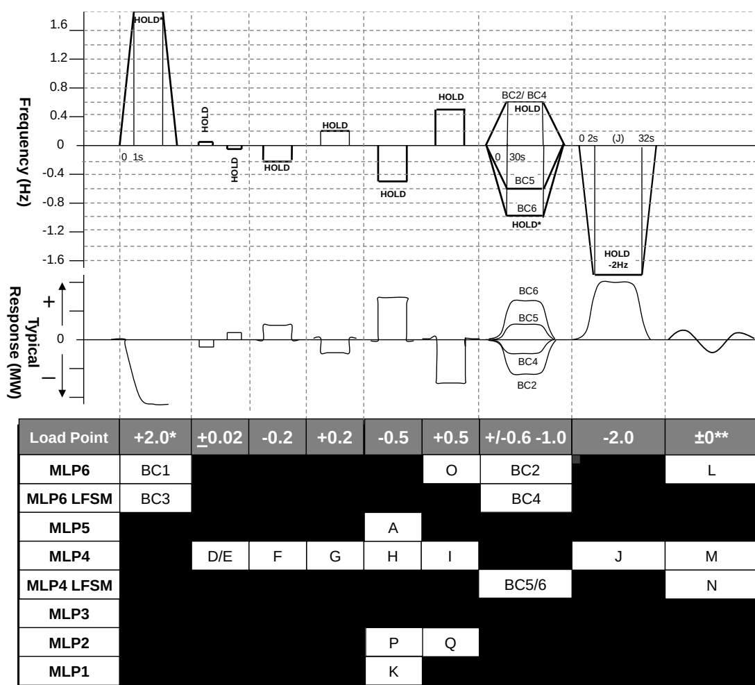
Figure C.8.1: Frequency Response Capability LFSM-O, LFSM-U, FSM Step
