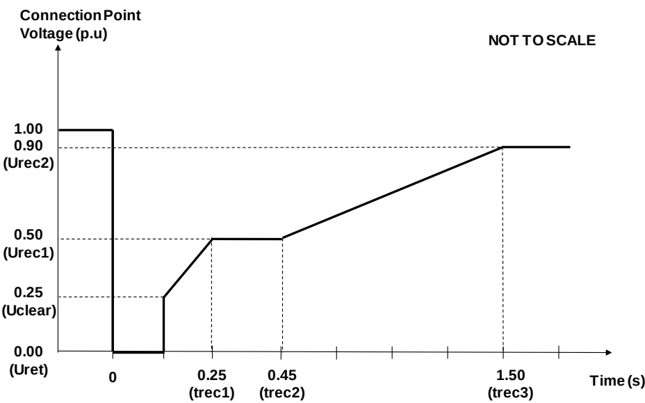
Figure 13.8 - Voltage against time curve applicable to Type D Synchronous Power Generating Modules connected at or above 110 kV
