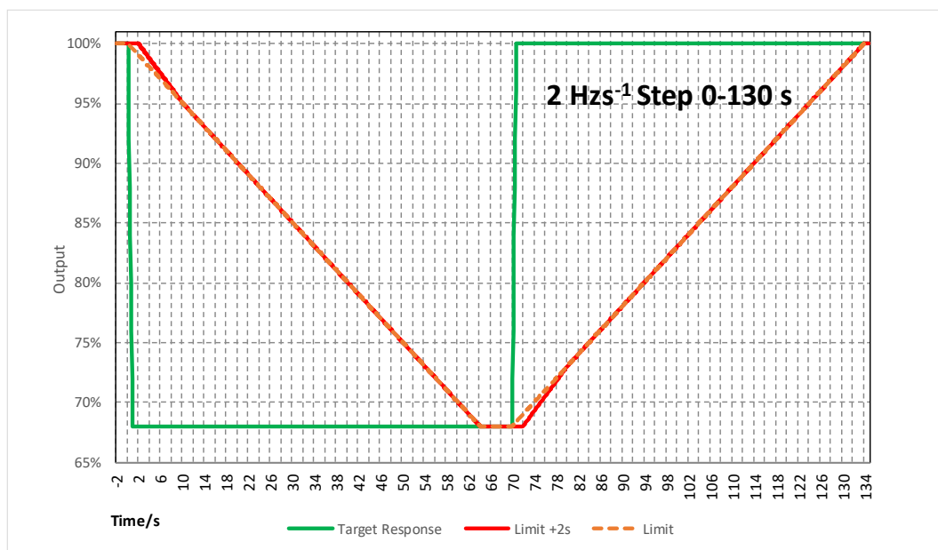
Figure B.6.1(ii): LFSM-O step response test – target response and limits
