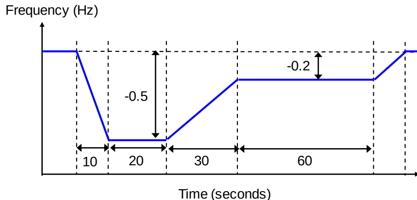
Figure C.7.4 Controller simulation
