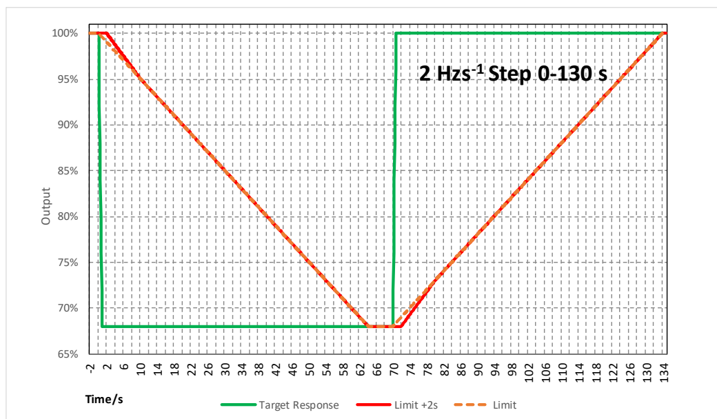
Figure B.5.1(ii): LFSM-O step response test – target response and limits
