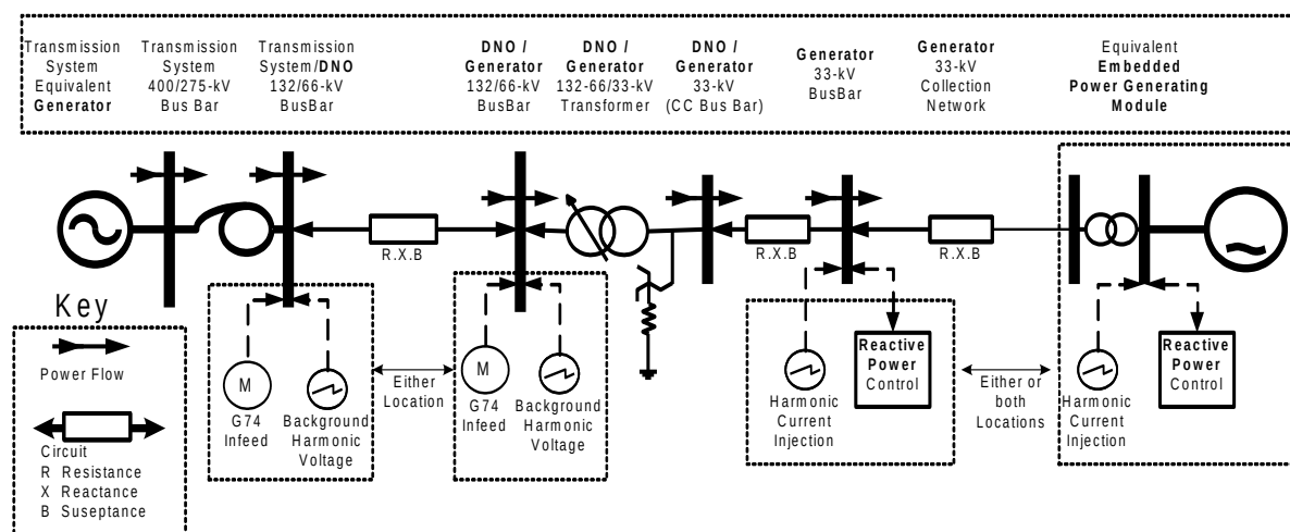
Figure 6.13 Example equivalent Total System representation
