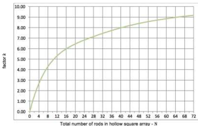
Figure B.1 — factor k for formula R5
