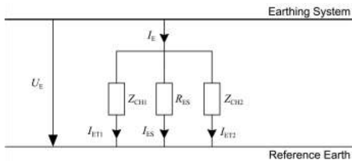
Figure 2 — Equivalent circuit for analysis
