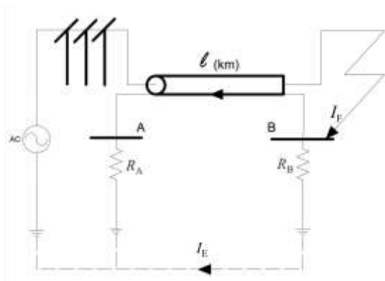
Figure D.3 — Line-cable circuit, remote source, fault at cable end
