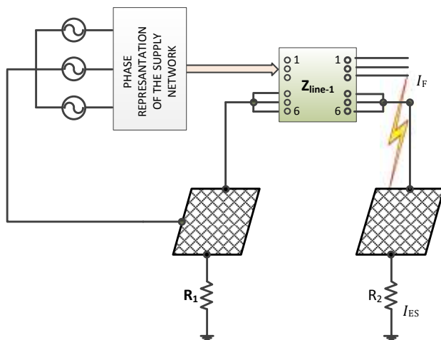
Figure H.2 — Circuit used for analysis purposes
