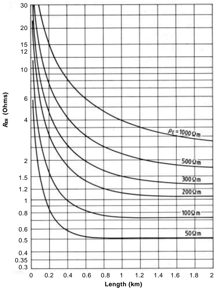
Figure F.1 — Resistance of long horizontal electrode (taken from BS EN 50522)
