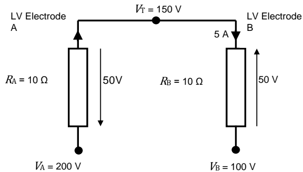
Figure I.1 — Example 1: Two electrodes of equal resistance
