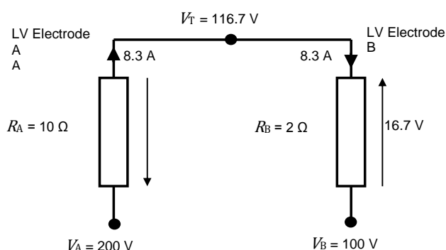
Figure I.2 — Example 2: Two electrodes of unequal resistance
