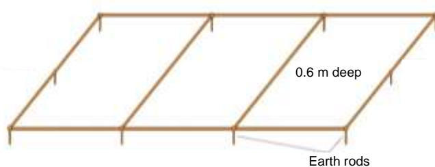
Figure 7 — Substation B basic earth grid and rods
