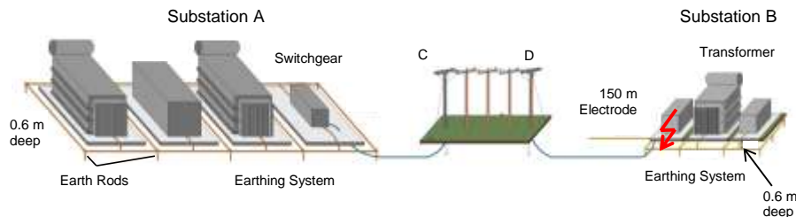
Figure 10 — Case study 3: Supply arrangement
