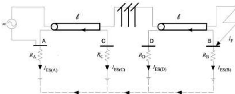
Figure 11 — Case study 3: Equivalent circuit
