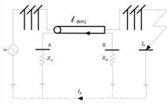
Figure D.4 — Line-cable-line circuit, remote source, remote fault
