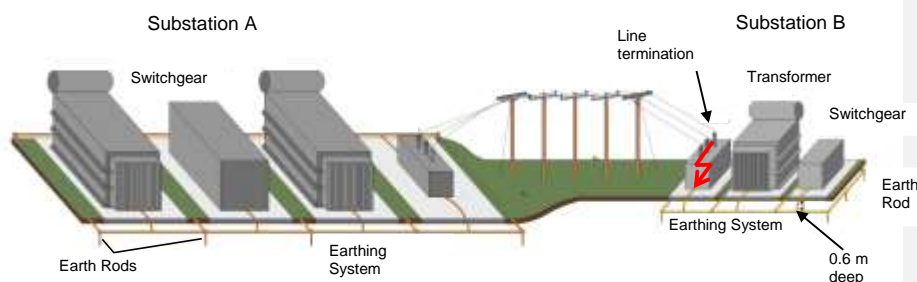
Figure 5 — Case study 1: Supply arrangement
