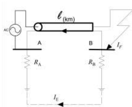
Figure D.1 — Cable circuit, local source, fault at cable end
