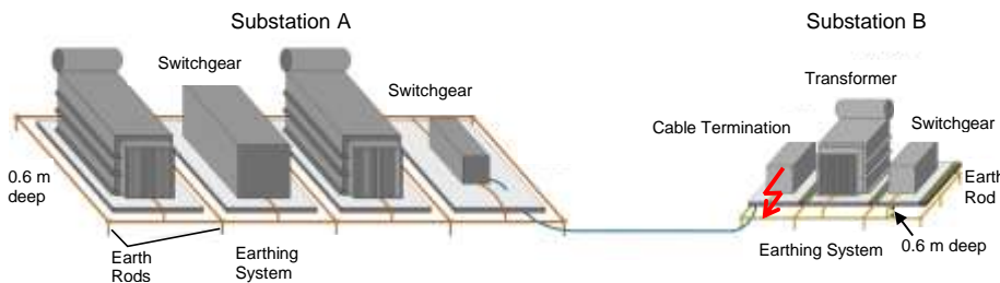
Figure 9 — Case study 2: Supply arrangement
