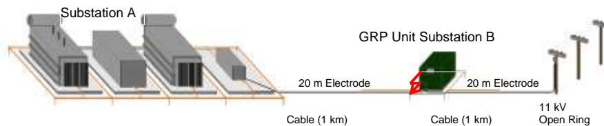
Figure 14 — Case study 5: Option 2
