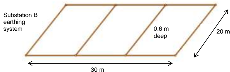
Figure 6 — Substation B basic earth grid
