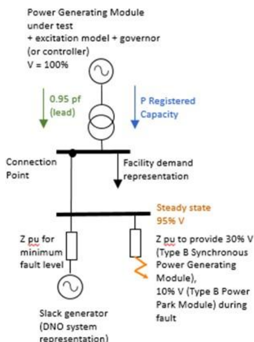
Figure 14: Example of Type B PGM Fault Ride Through and Fast Fault Current Injection Studies.
