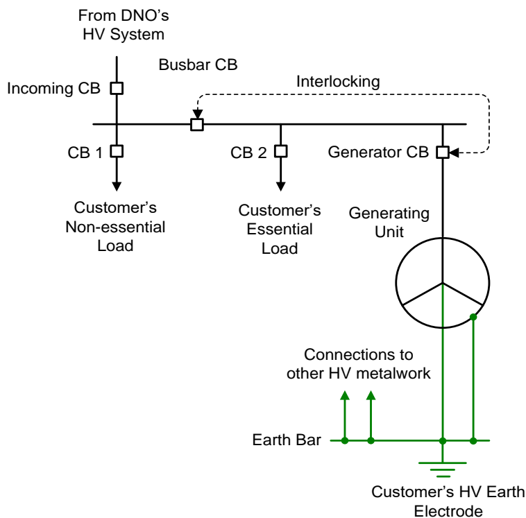
Figure 8.1 - Typical Earthing Arrangement for an HV Generating Unit Designed for Independent Operation (ie Standby Operation) Only
